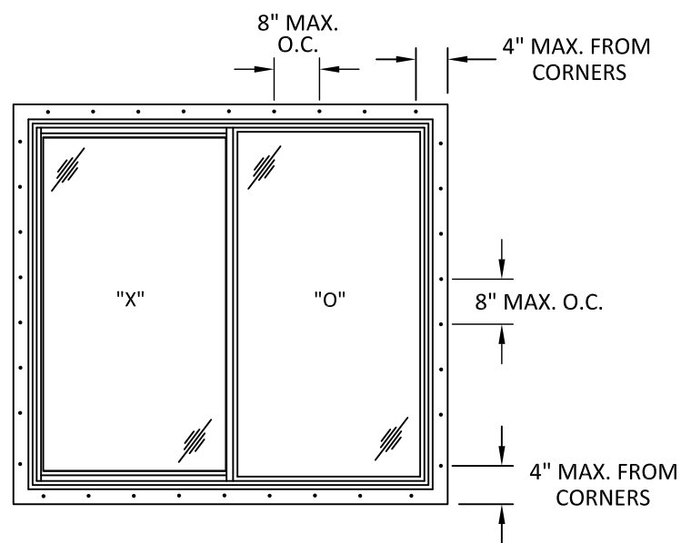
TYPICAL ANCHOR LAYOUT NAIL FIN INSTALLATION
